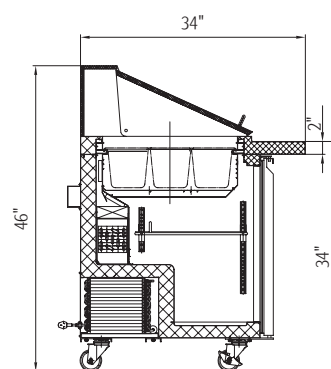
Side Section
