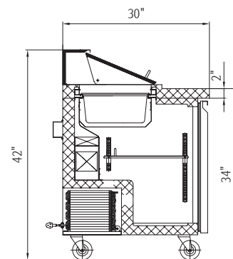
Side Section
