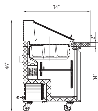
Side Section
