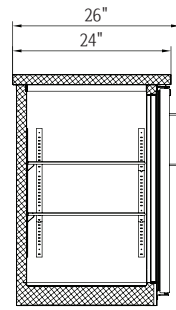
Side Section
