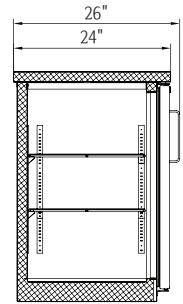
Side Section
